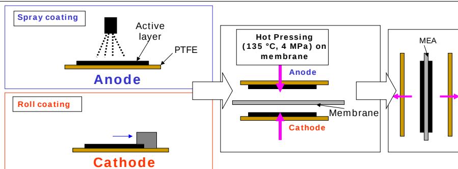
Figure 3: transfer method to synthesize MEA
