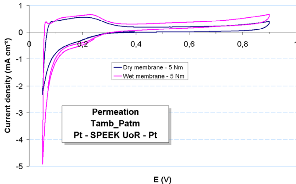
Figure 2: LSV at 25^\circ \text{C} obtained for SPEEK membrane
