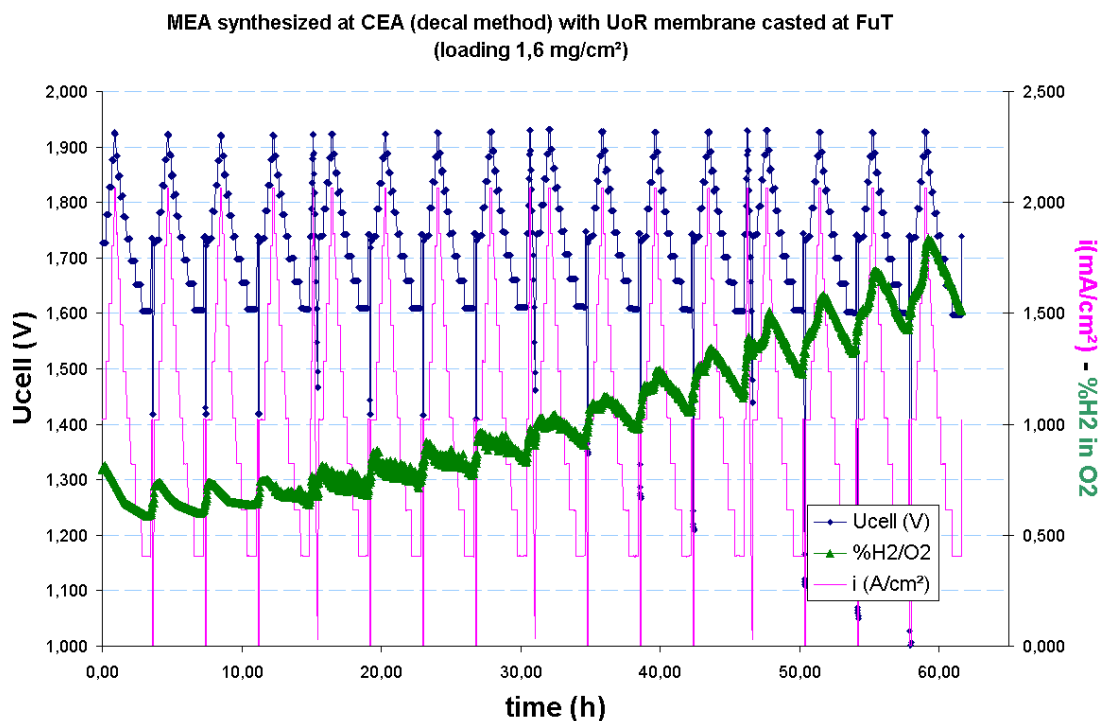
Figure 6: evolution of parameters ( U , I , gas purity) vs. time for MEA n°2 at 60°C
