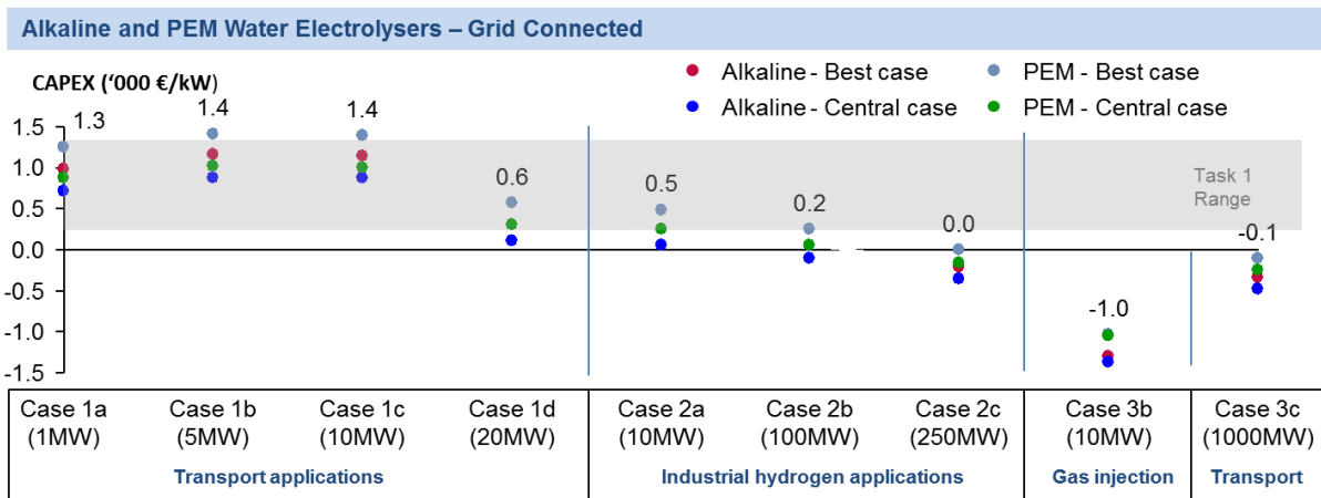
Figure 16: Capex targets for Alkaline and PEM technologies required to compete with counterfactual in Germany, 2030.
