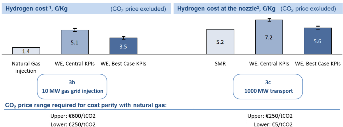
Figure 15: Hydrogen cost at the point of use for energy storage applications in Germany, 2030.
