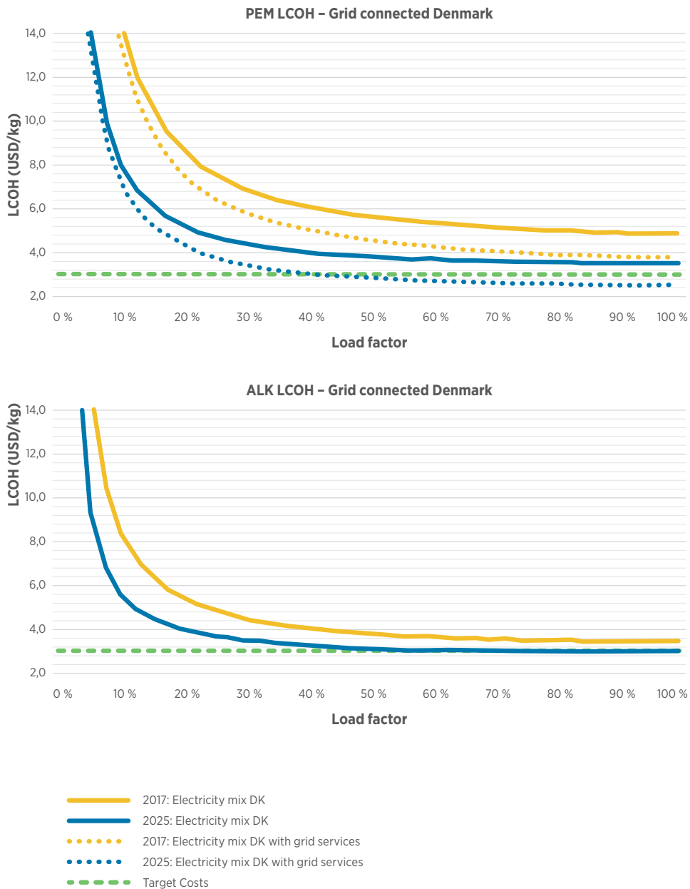
Figure 9: Levelised cost of hydrogen (LCOH) produced via ALK and PEM in 2017 and as expected in 2025
