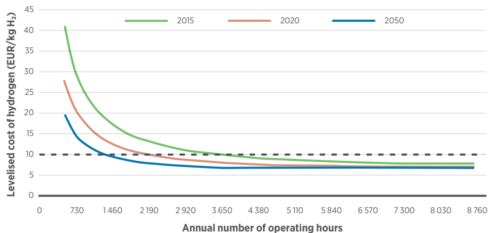
Figure 10: LCOH vs. operating time (HRS for buses)
