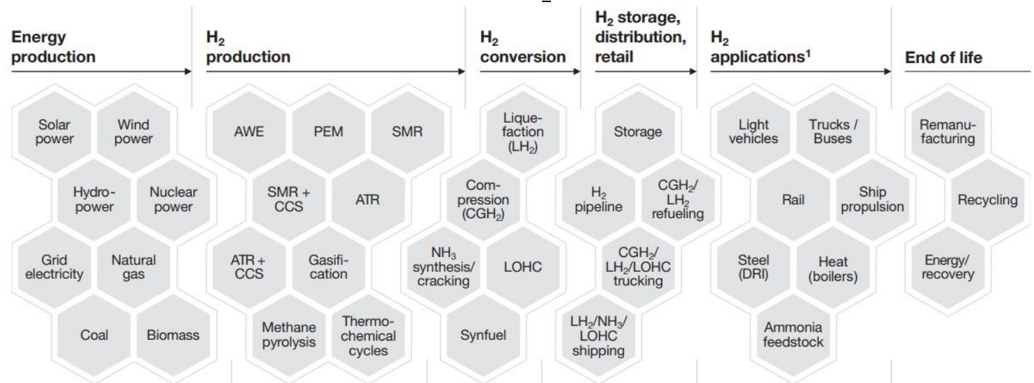
Hydrogen production pathways and associated steps in upstream and downstream the value chain with embedded CO 2 emissions 1
