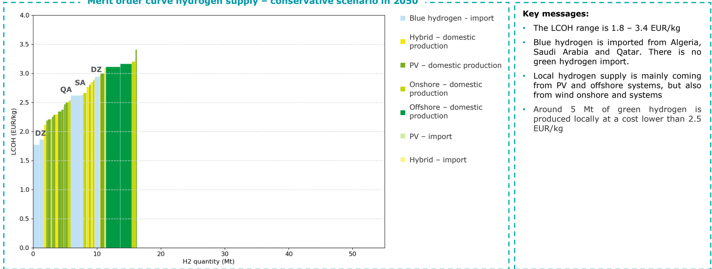
Merit order curve hydrogen supply – conservative scenario in 2050
