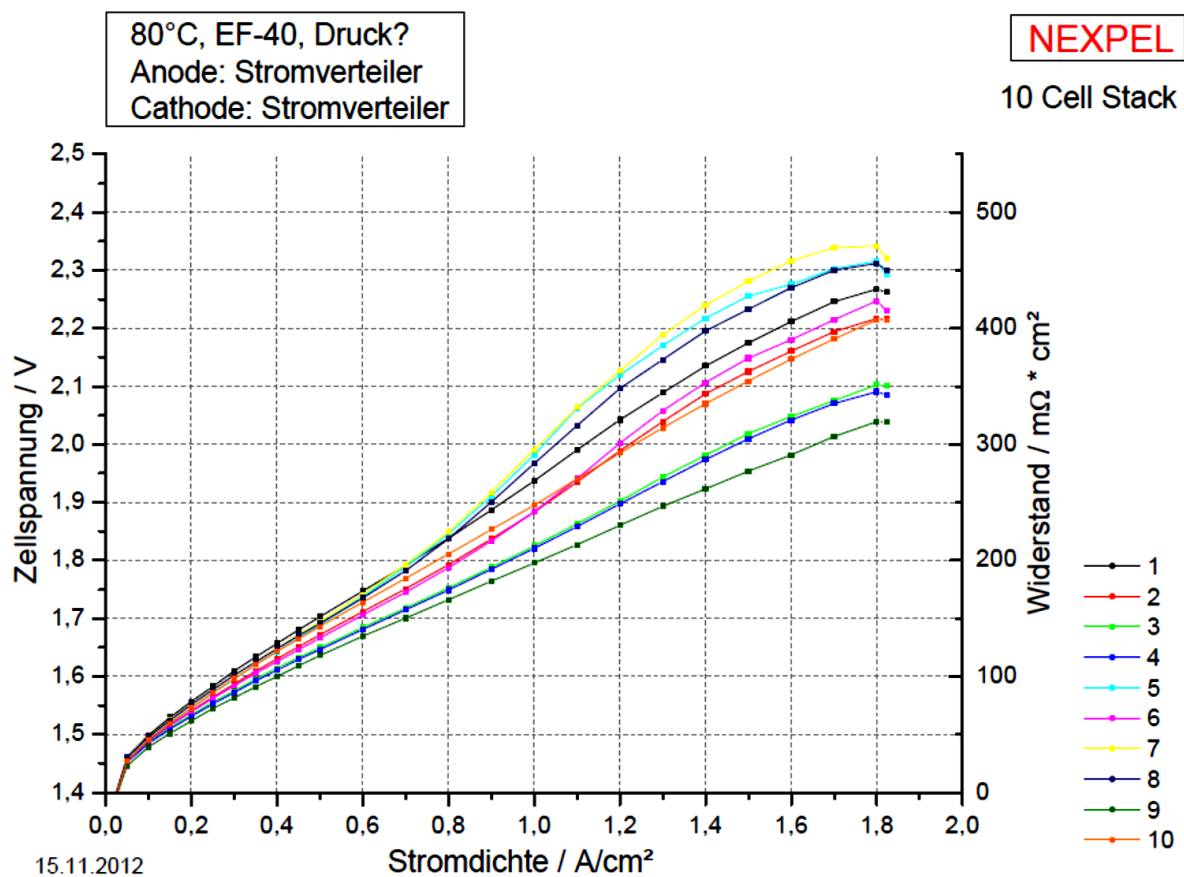
Figure 3: Single cells performance after 20 hours of conditioning
