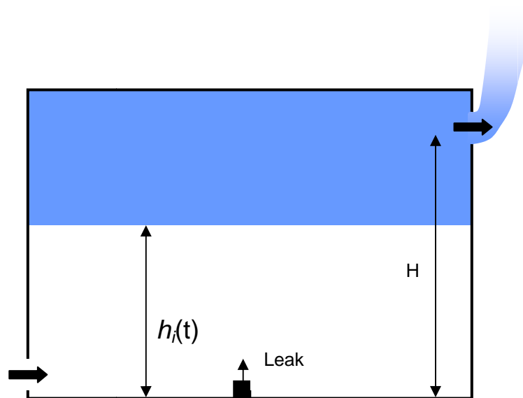
Figure 15. Schematics of the displacement regime obtained in case of natural ventilation by two openings.
