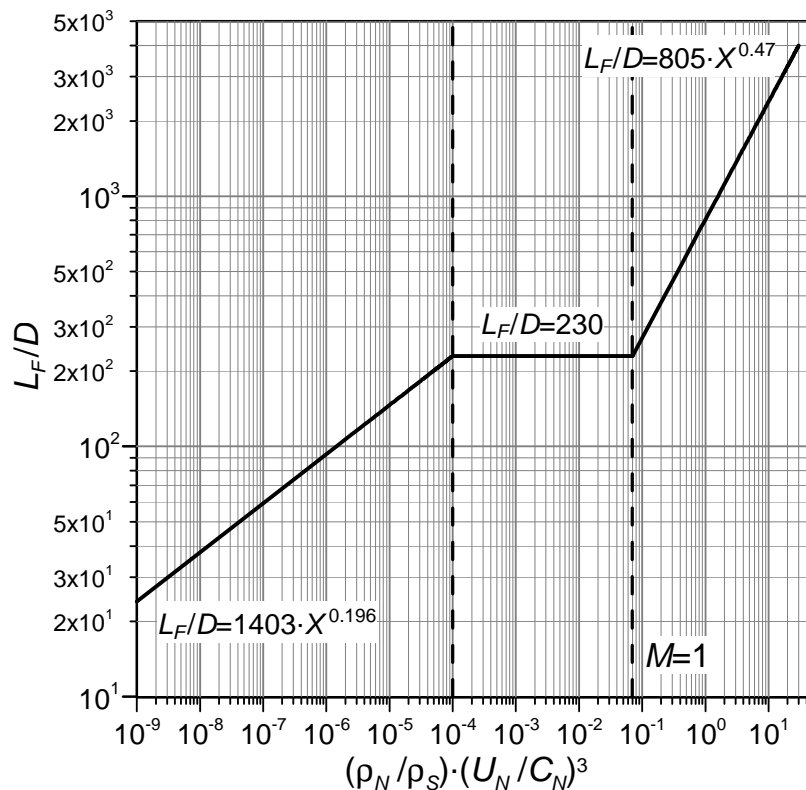
Figure 24. Dimensionless flame length correlation (Molkov and Saffers, 2013).
