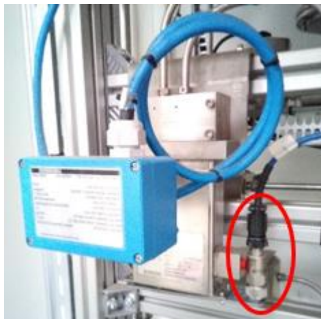
Figure 20 : ATEX accelerometer
