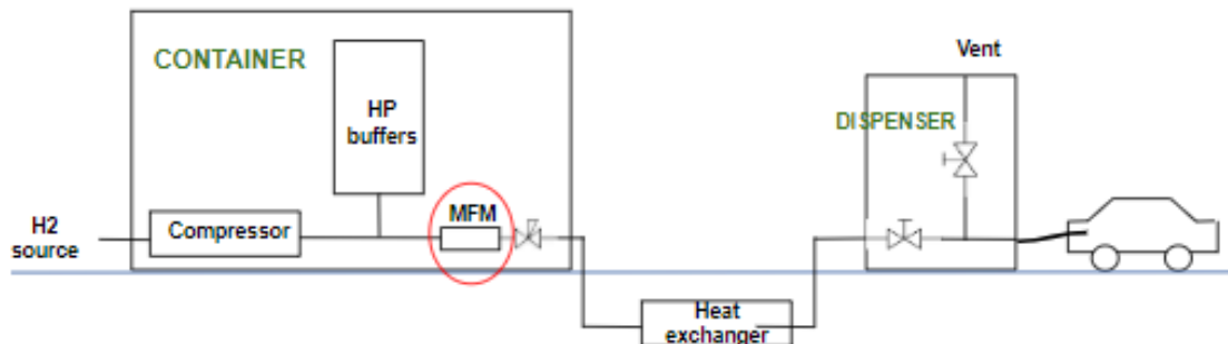
Figure 6: Illustration of Configuration 1, where the MFM is located in the main container
