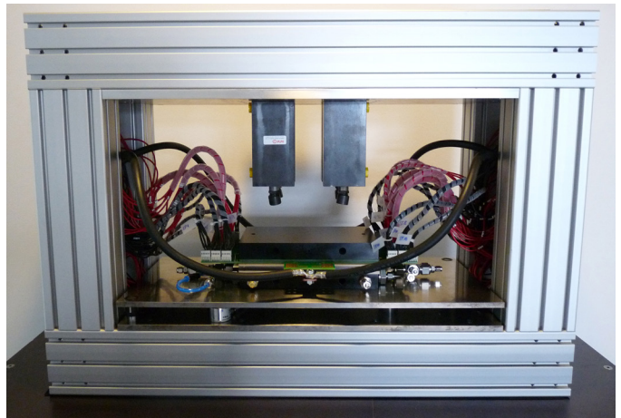
First version of a segmented graphitic test cell (top, 200 cm 2 active area) with contact pins and cell housing with compression unit and electrical cell contacts for the integration of the segmented cell (bottom).
