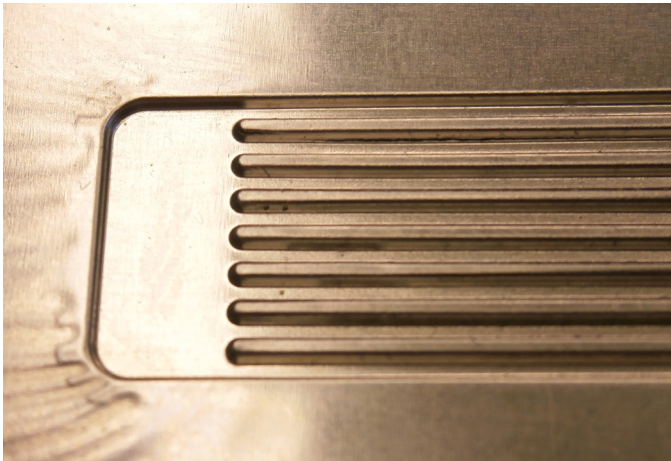
Result after first stamping test of small-scale single cell test plate.
