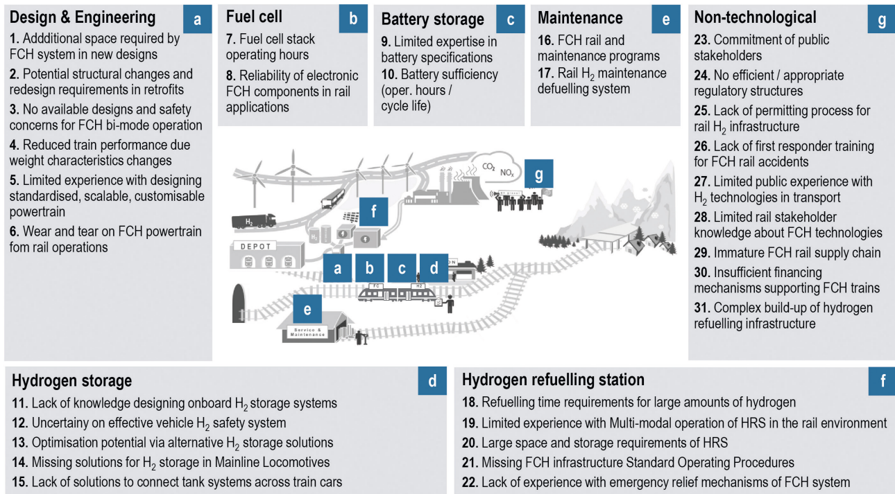
Figure 9: Barriers to FCH technology in the railway environment.
